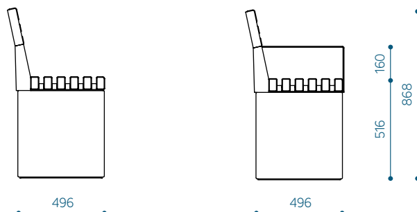
Tahu bench, with backrest and armrests- TAHB200
