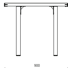
Klaar Steel small table- KLST90
