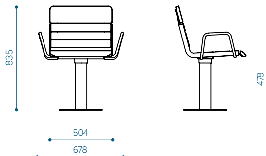
Hula chair, with 2 armrests - HUB50-02
