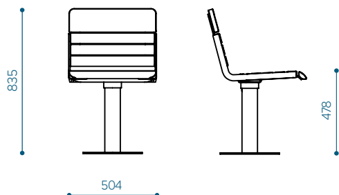
Hula chair, without armrests - HUB50
