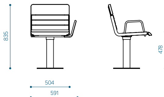
Hula chair, with left armrest - HUB50-05
