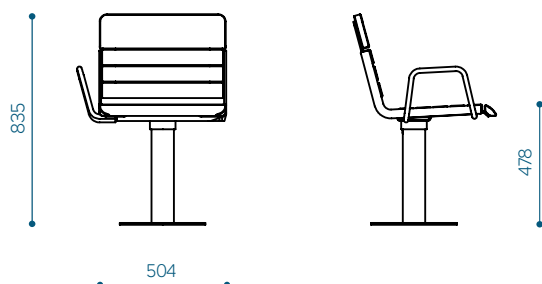
Hula chair, with right armrest - HUB50-04
