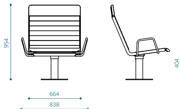
Hula lounge chair, high backrest, with 2 armrests - HUC60-02
