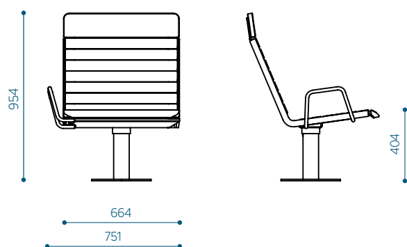
Hula lounge chair, high backrest with right armrest - HUC60-04
