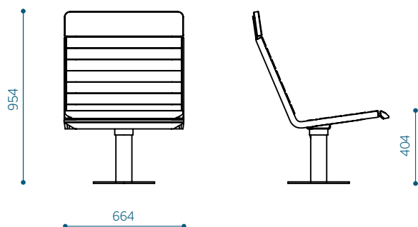
Hula lounge chair, high backrest, without armrests - HUC60
