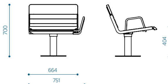
Hula lounge chair, with left armrest - HUB60-05
