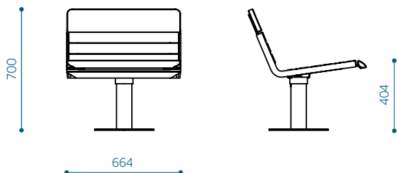
Hula lounge chair, without armrests - HUB60
