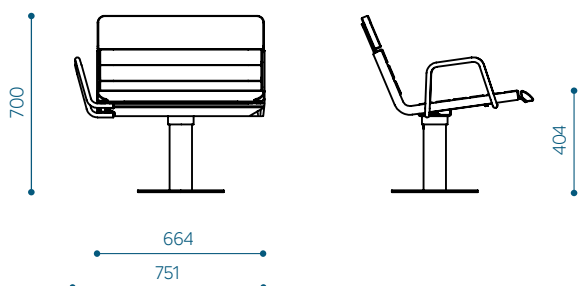
Hula lounge chair, with right armrest - HUB60-04
