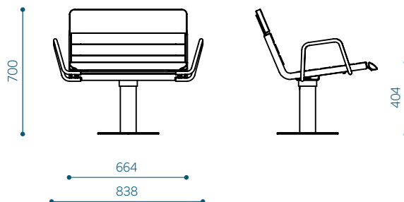
Hula lounge chair, with 2 armrests - HUB60-02
